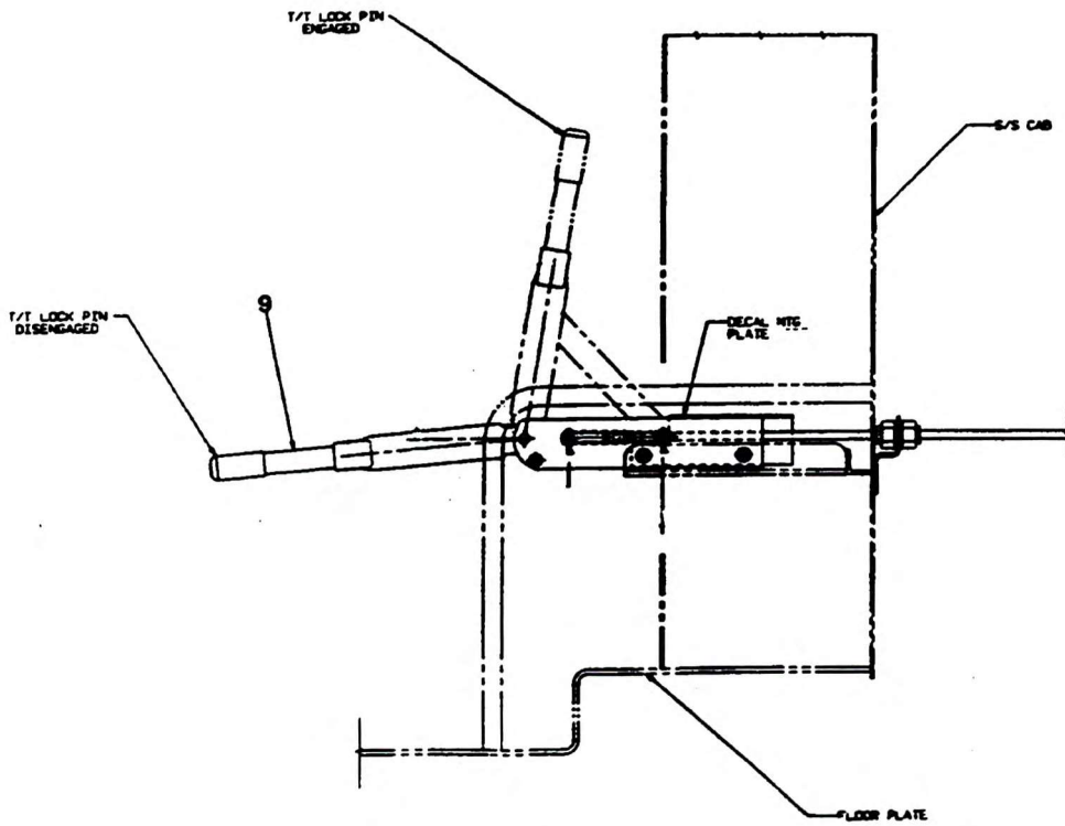
PARTIAL VIEW OF OPERATORS CAB
